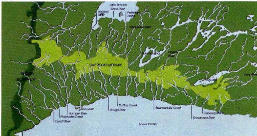
Figure 2: Location of the Oak Ridges Moraine
