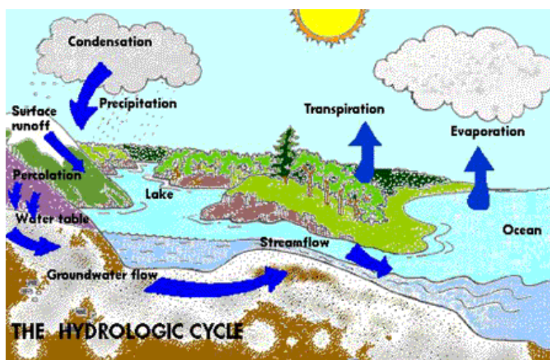
Figure 1: The Hydrologic Cycle (Source: Environment Canada, The Hydrologic Cycle )
